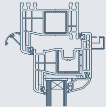
PCV frame
